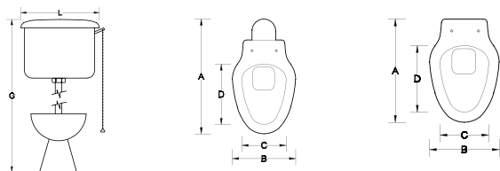
Front View ("S" Trap & "P" Trap)
