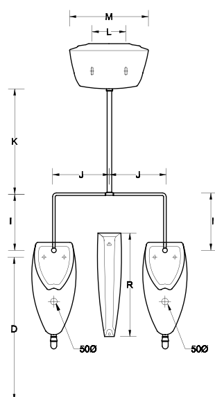
Front View (Jumeriah Exposed Urinal)
