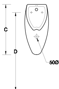
Front View (Jumeriah Concealed Urinal)
