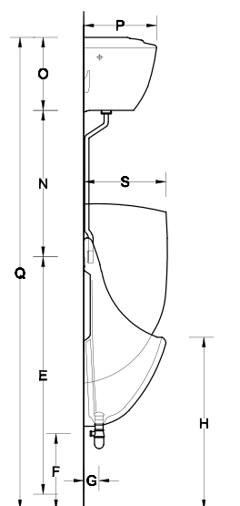
Side View (Jumeriah Exposed Urinal)
