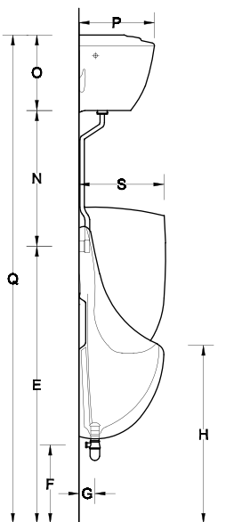
Side View (Vitara Exposed Urinal)
