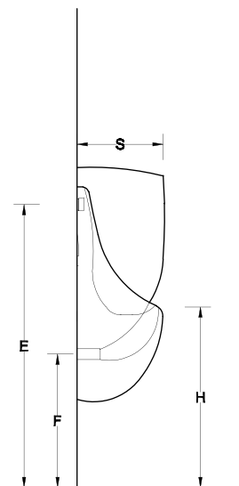
Side View (Vitara Concealed Urinal)
