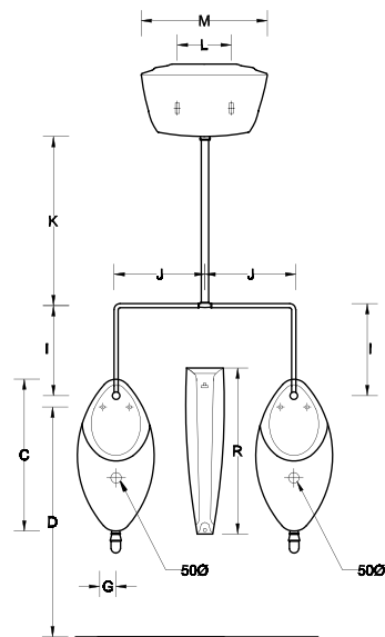
Front View (Vitara Exposed Urinal)
