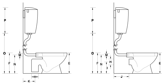
Side View ("S" Trap)
