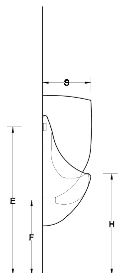
Side View (Jumeriah Concealed Urinal)
